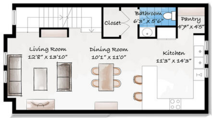
Main Level
